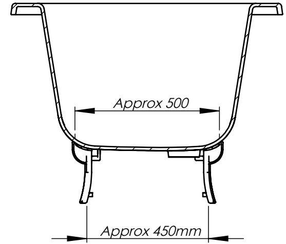
PROFILE B-B
